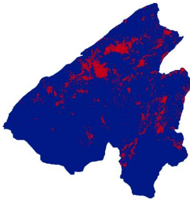
forest / non-forest
