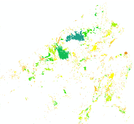
isolation
