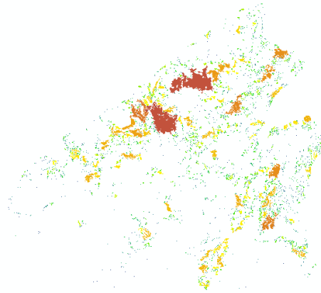
patch area
