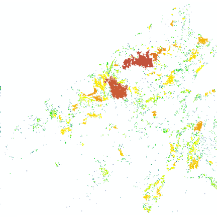
perimeter:area
